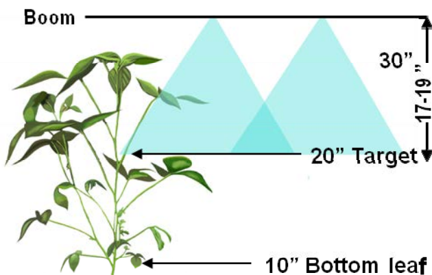
Figure 1. Height adjustment for a spray boom equipped with 80 degree flat fan nozzles spaced at 20" and used in 30" tall soybeans
